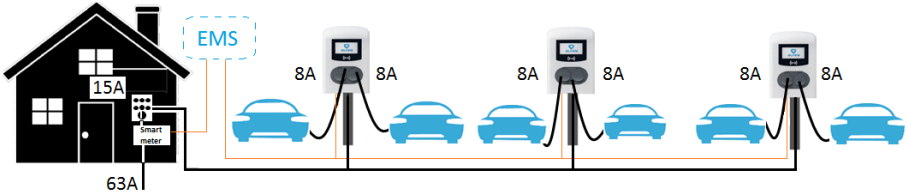
Figure 5.9: Scenario ALB in combination with smart energy meter, EMS and multiple charging stations
