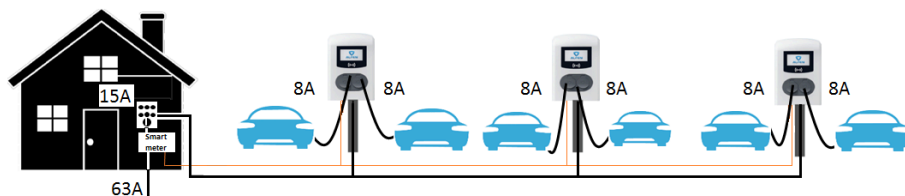
Figure 5.7: Scenario ALB in combination with smart energy meter and multiple charging stations
