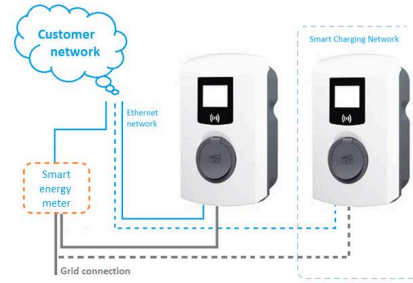
Figure 5.3: Active Load Balancing with energy meter (Modbus TCP/IP)
