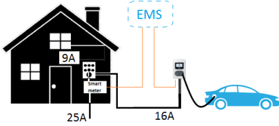
Figure 5.8: Scenario ALB in combination with Smart energy meter and EMS
